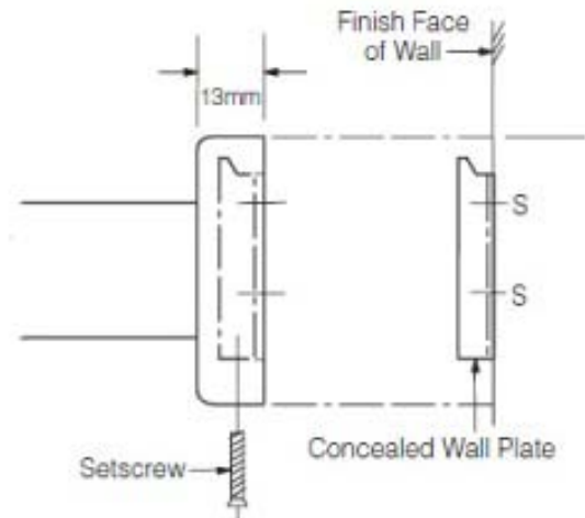
Rear View of Cover Flange & Mounting Arm, showing position of Concealed Wall Plate (Note Set-screw)
